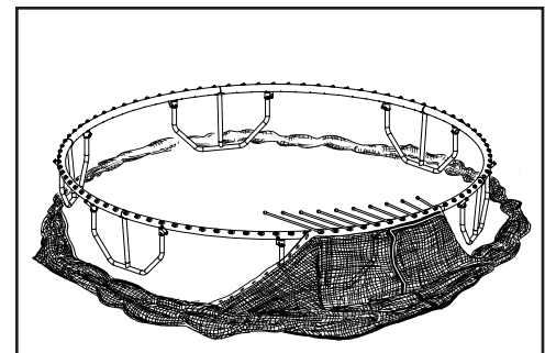
Figure 10: Inserting the remaining rods
