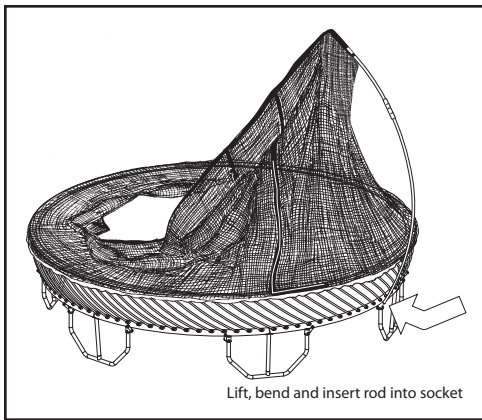
Figure 19: Inserting an enclosure rod into a socket
